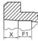
Welding relief
